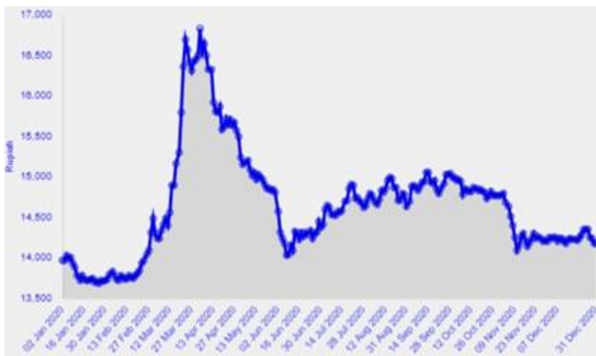
Gambar 1. Kurs transaksi ( exchange rates on transaction ) - USD
